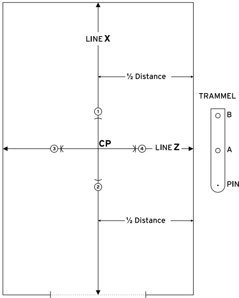
Figure 6 Marking out straight tiling
