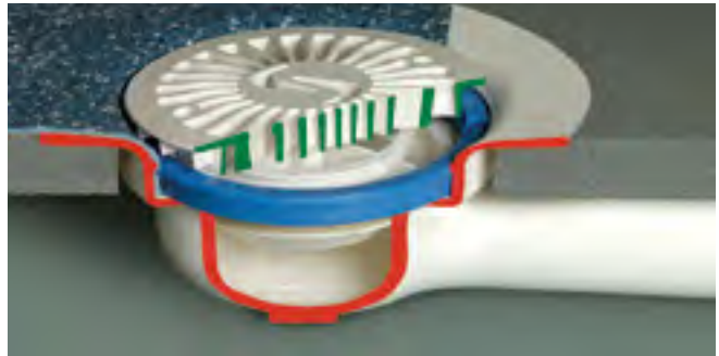
Figure 2 Drain with clamping ring in place
