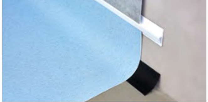
Figure 10 Fitting to Ceramic tiles
