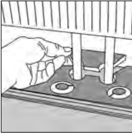
Figure 31 Radiator pipes
