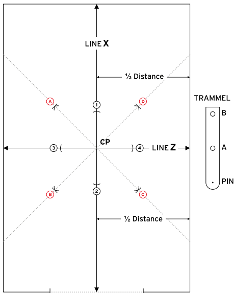
Figure 7 Marking out diagonal tiling
