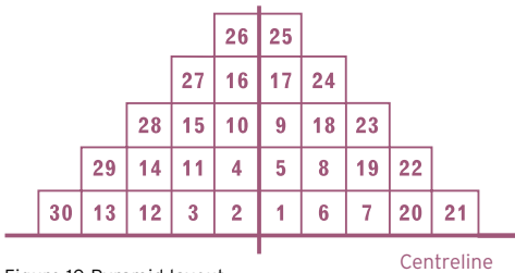
Figure 10 Pyramid layout
