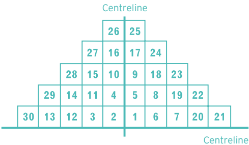
Figure 9 Pyramid layout
